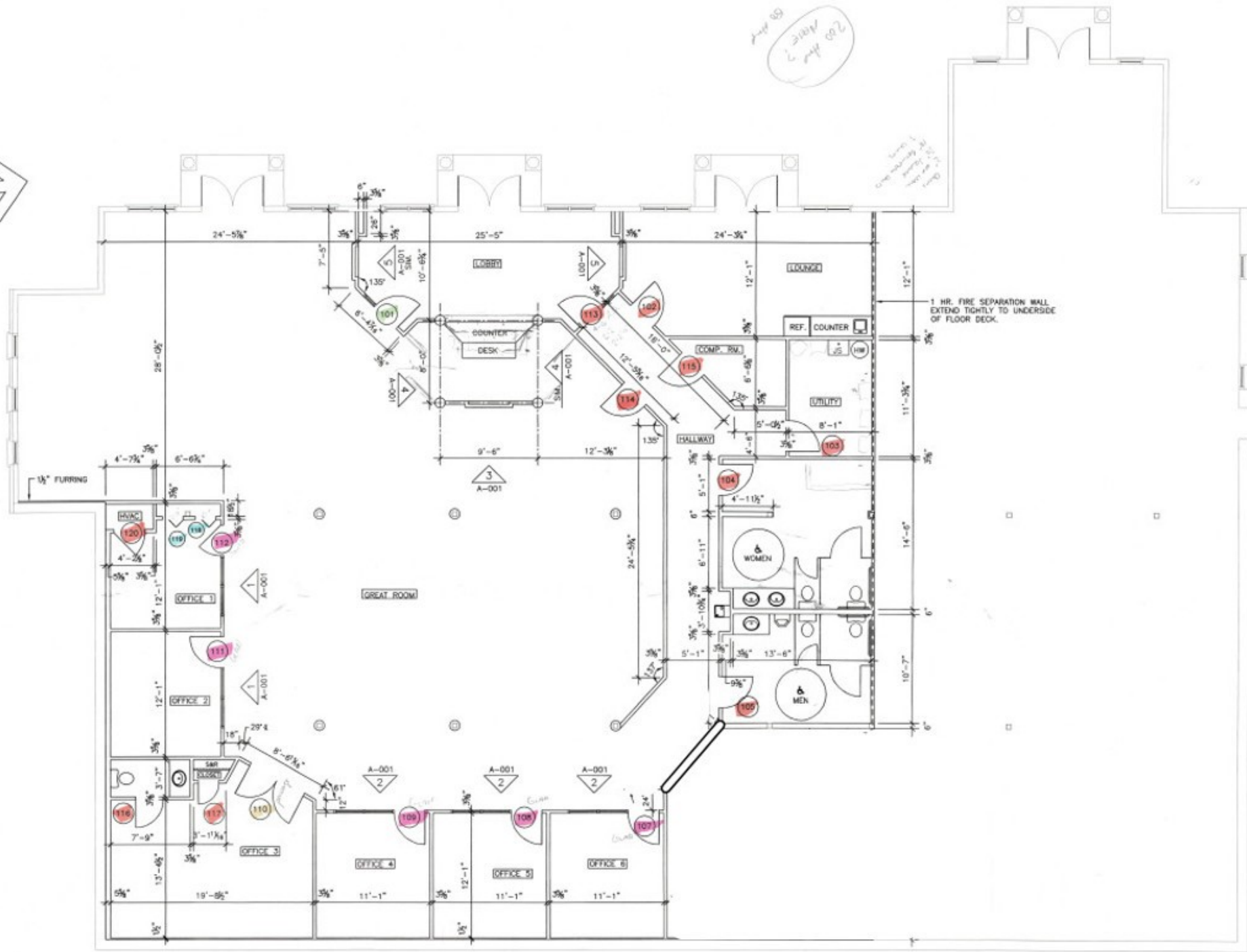
1 FLOOR PLAN A-101 3/16" = 1'-0"
